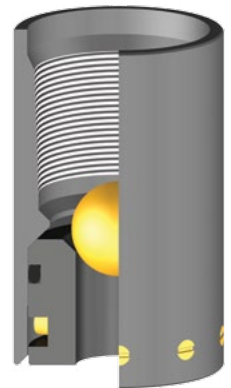
Pump-Out Plug w/ Shear Screws and Ball Seat
